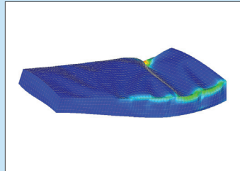
Buckling
