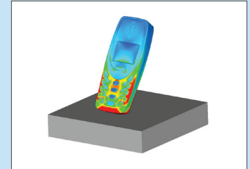
Automated Impact Analysis (AIA™) and Drop Test
