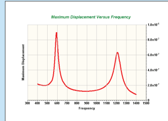
Frequency Response
