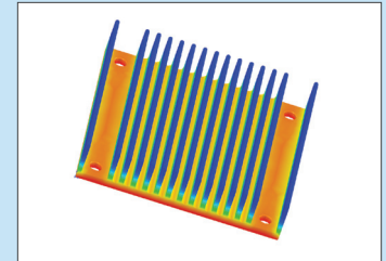
Nonlinear Steady State and Transient Heat Transfer
