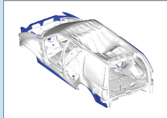
Normal Modes
